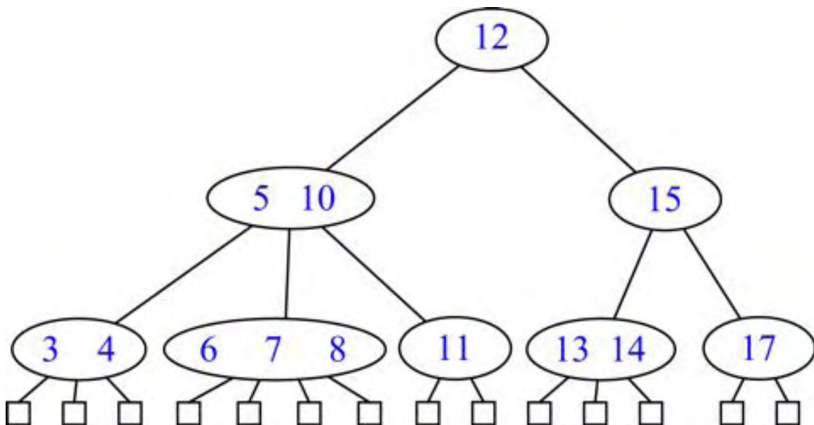
Figure 10.20: A (2,4) tree.
