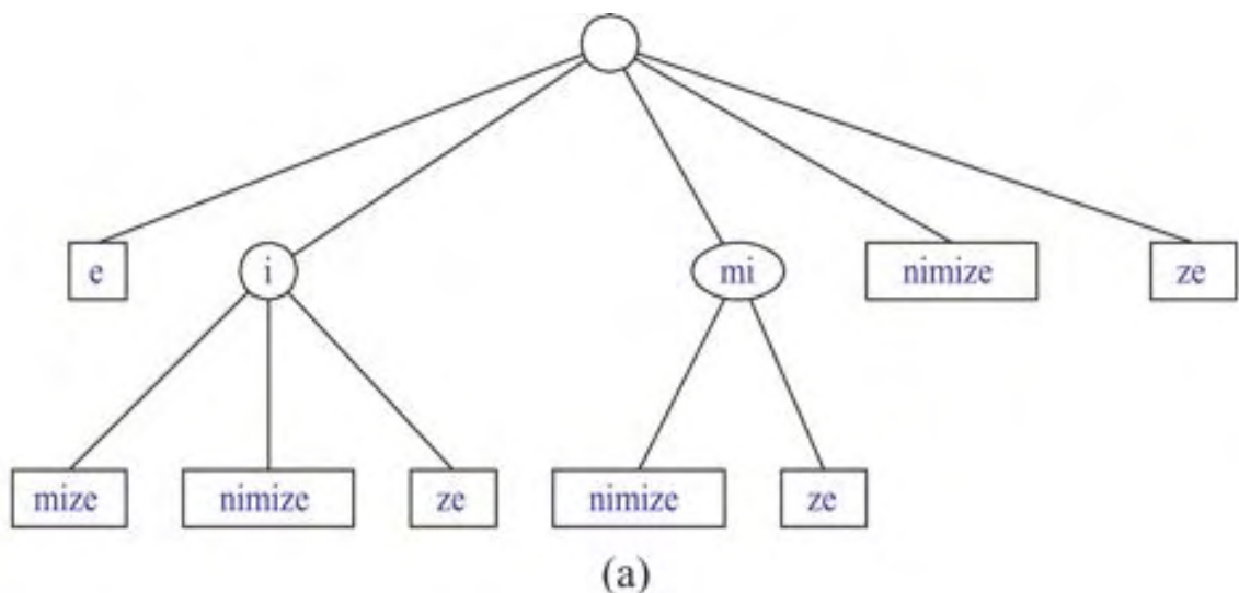
Figure 12.10: (a) Suffix trie T for the string X = "minimize". (b) Compact representation of T , where pair (i,j) denotes X[i..j] .
