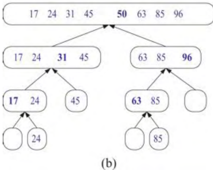
Figure 11.10: Visualization of quick-sort. Each node of the tree represents a recursive call. The nodes drawn with dashed lines represent calls that have not been made yet. The node drawn with thick lines represents the running invocation. The empty nodes drawn with thin lines represent terminated calls. The remaining nodes represent suspended calls (that is, active invocations that are waiting for a child invocation to
