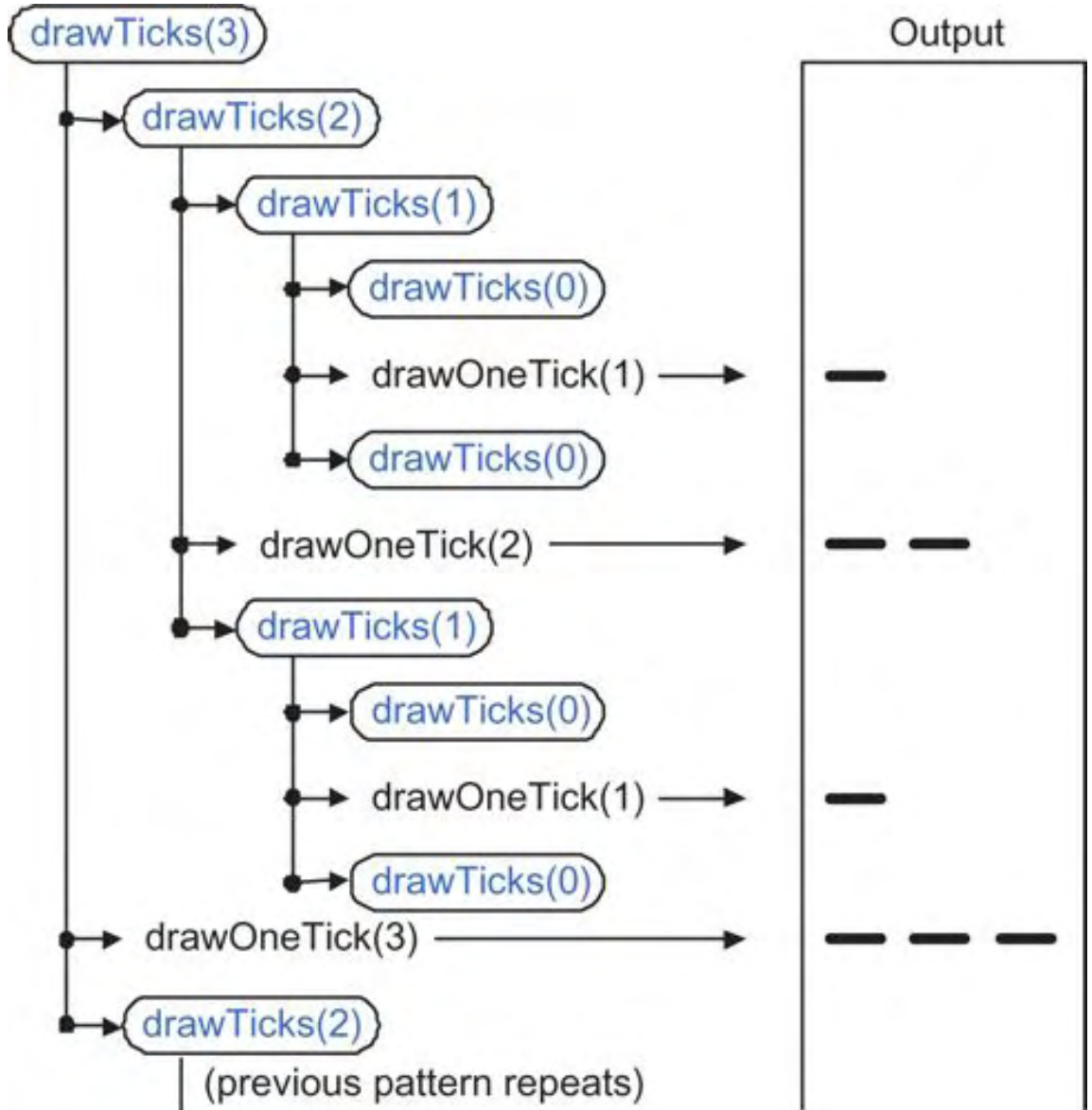
Figure 3.23: A partial recursion trace for the call drawTicks(3) . The second pattern of calls for drawTicks(2) is not shown, but it is identical to the first.
