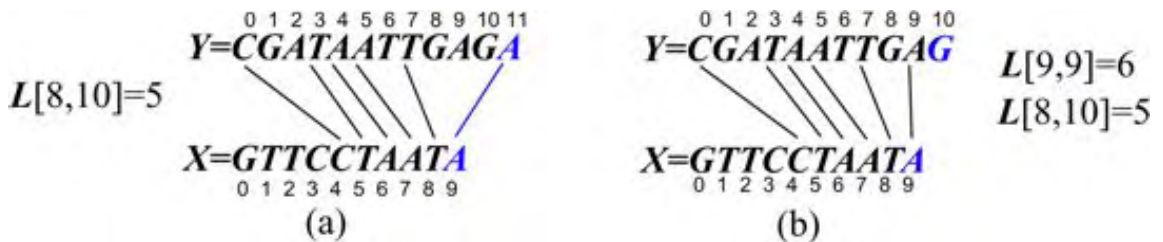
Figure 12.12: The two cases in the longest common subsequence algorithm: (a) x_i = y_j ; (b) x_i \neq y_j . Note that the algorithm stores only the L[i,j] values, not the matches.
