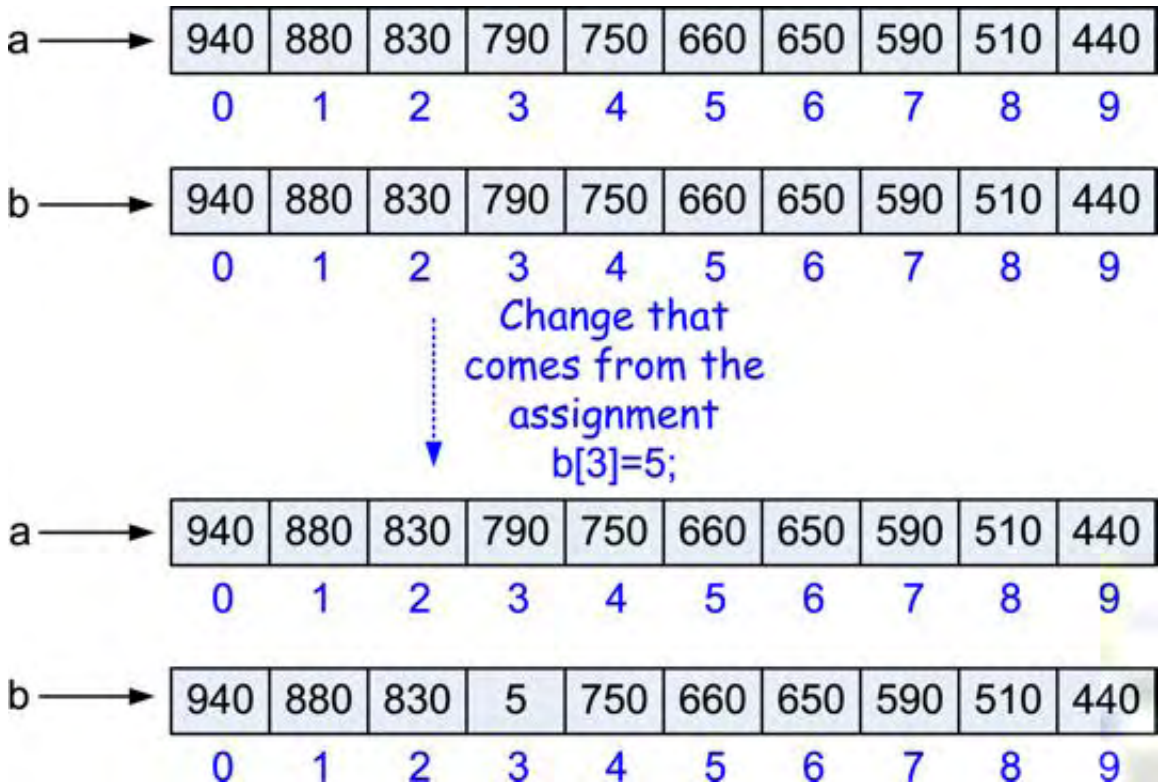
Figure 1.8: An illustration of cloning of array objects. We show the result of setting " b[3] = 5; " after previously setting " b = a.clone(); ".
