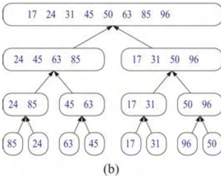
Figure 11.2: Visualization of an execution of merge-sort. Each node of the tree represents a recursive call of merge-sort. The nodes drawn with dashed lines represent calls that have not been made yet. The node drawn with thick lines represents the current call. The empty nodes drawn with thin lines represent completed calls. The remaining nodes (drawn with thin lines and not empty) represent calls that are waiting
