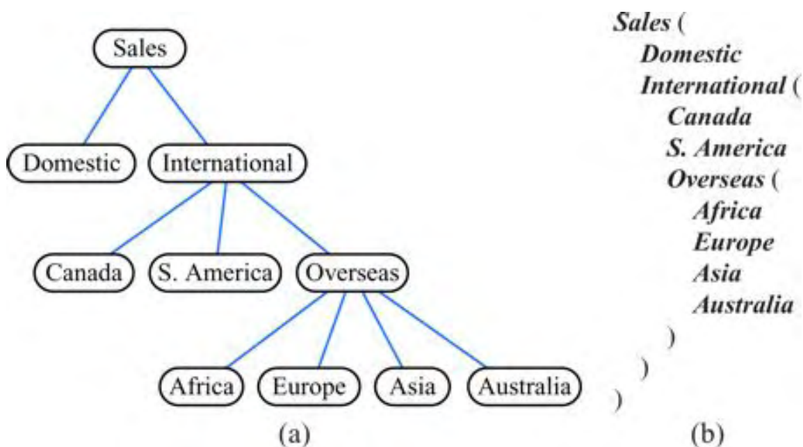
Figure 7.21: (a) Tree T ; (b) indented parenthetical representation of T .
