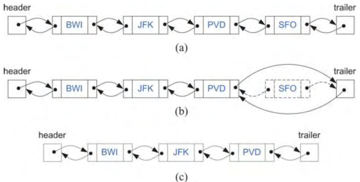
Figure 3.15: Removing the node at the end of a doubly linked list with header and trailer sentinels: (a) before deleting at the tail; (b) deleting at the tail; (c) after the deletion.
