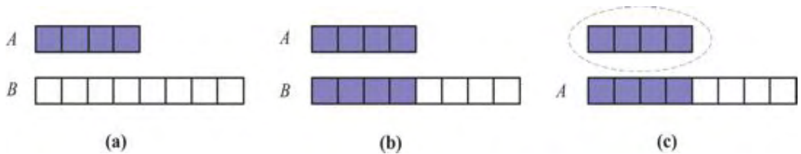
Figure 6.2: An illustration of the three steps for "growing" an extendable array: (a) create new array B ; (b) copy elements from A to B ; (c) reassign reference A to the new array. Not shown is the future garbage collection of the old array.
