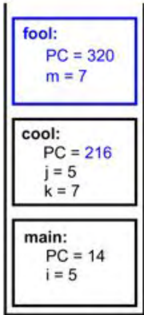
Java Stack
