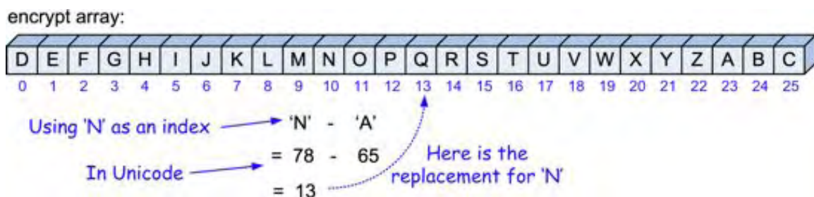
Figure 3.6: Illustrating the use of uppercase characters as array indices, in this case to perform the replacement rule for Caesar cipher encryption.
